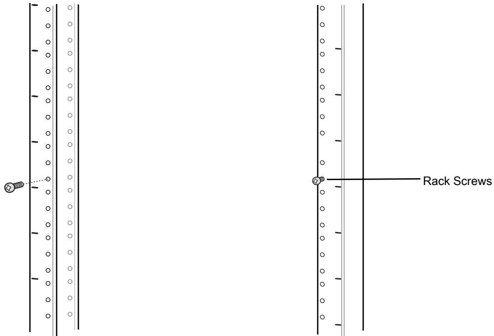
Figure 59 Install Rack System Screws
