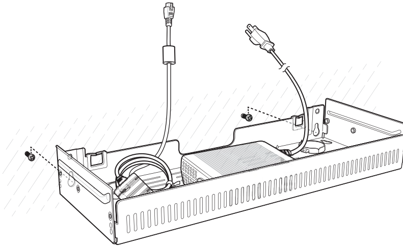
Figure 62 Horizontal Installation
