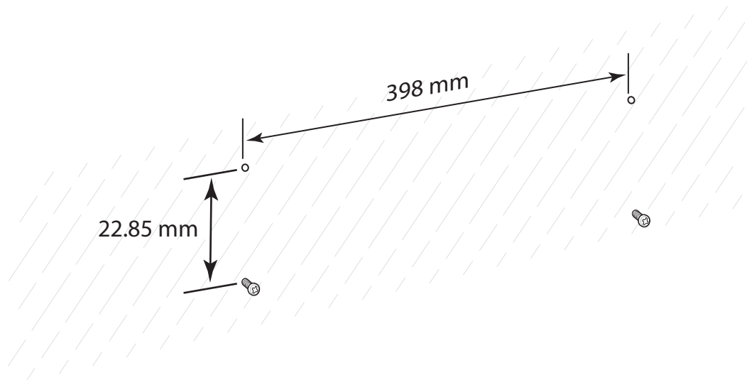
Figure 61 Horizontal Mounting Template
