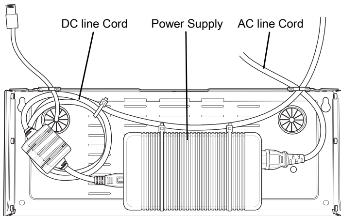
Figure 50 Power Supply in Bottom Tray
