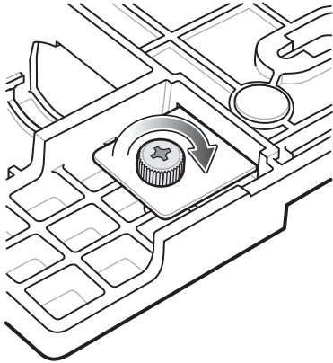
Figure 32 Secure Screw
