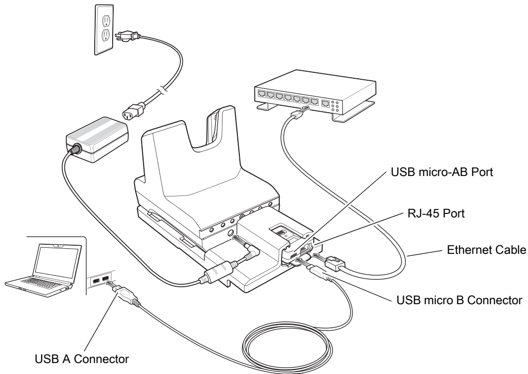
Figure 34 Ethernet Bracket Setup
