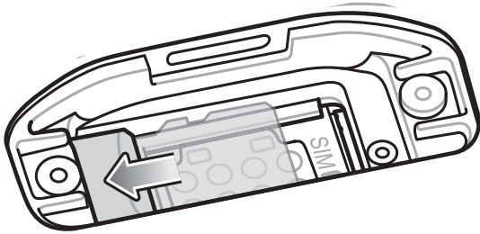
Figure 4 Push microSD Card into the SD Card Slot
