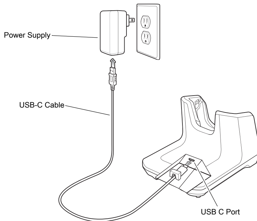
Figure 21 1-Slot Base Charge Only Cradle Setup
