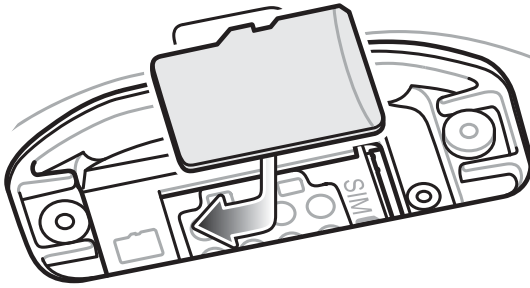
Figure 14 Align microSD Card
