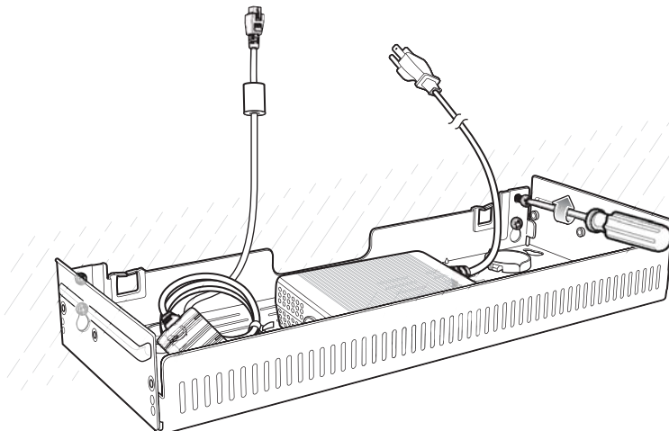
Figure 63 Horizontal Installation - Tighten Screws
