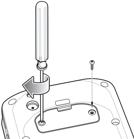
Figure 16 Secure Access Door
