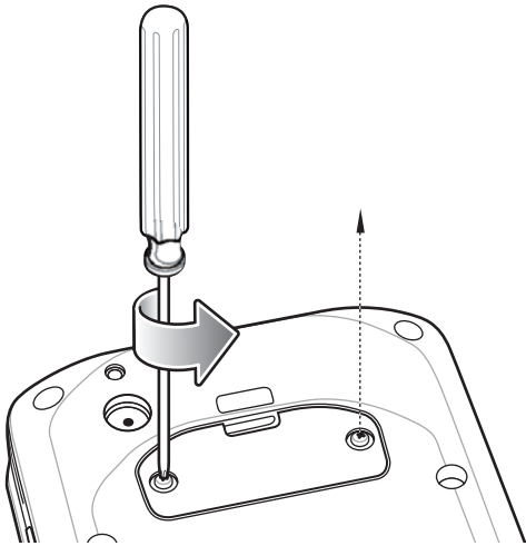
Figure 12 Remove Access Door
