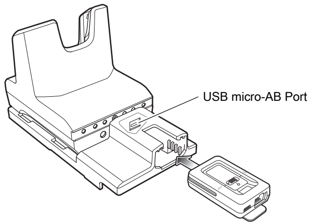
Figure 33 Insert Module
