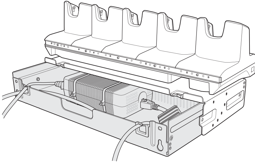
Figure 54 Slide Top Tray onto Bottom Tray
