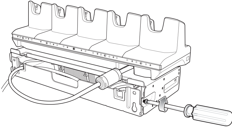
Figure 56 Secure Top and Bottom Tray
