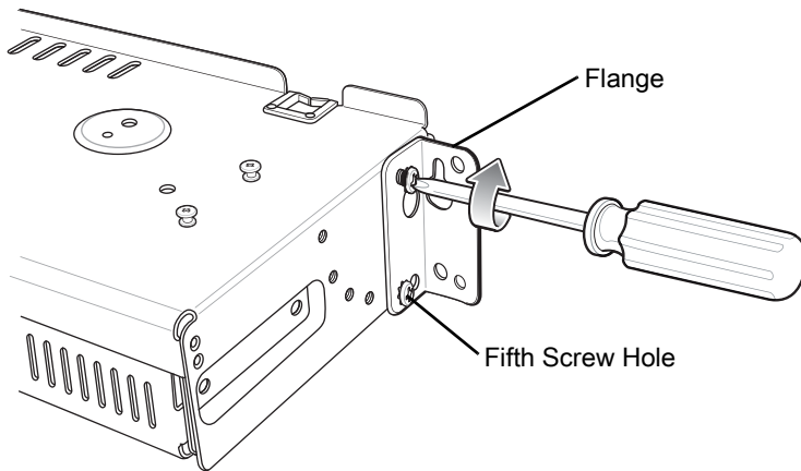
Figure 58 Flange 25° Position
