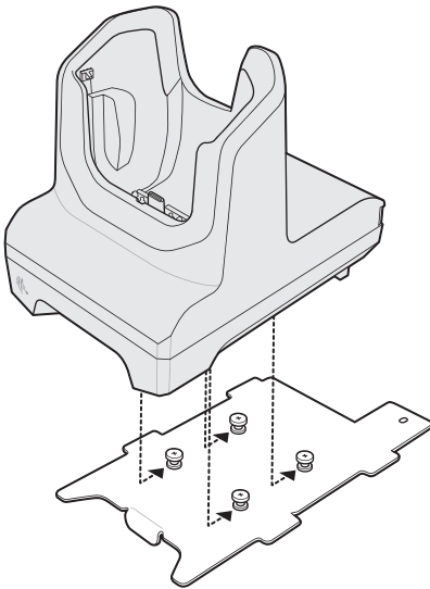
Figure 29 Align Cradle with Plate
