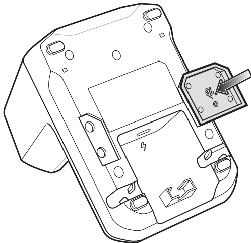
Figure 23 Align Mounting Bracket
