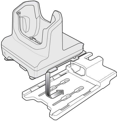
Figure 30 Align Cradle/Plate with Bracket
