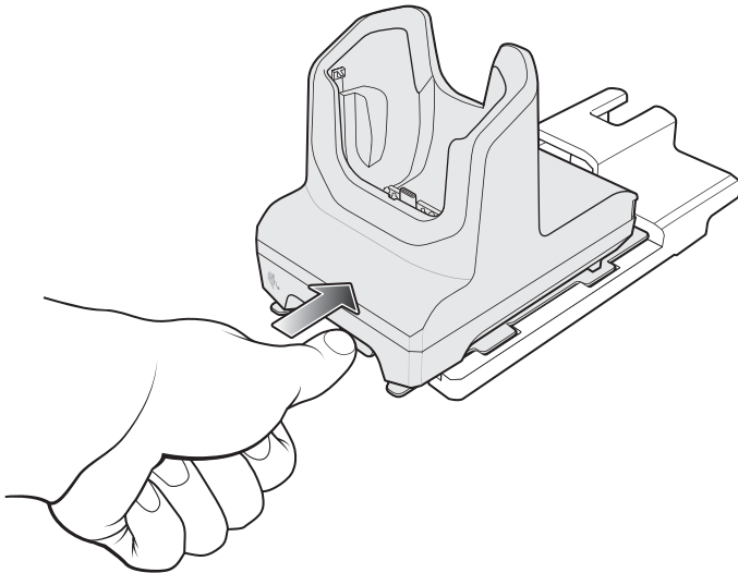
Figure 31 Push Plate into Bracket
