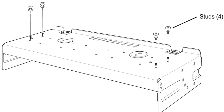
Figure 51 Install Studs
