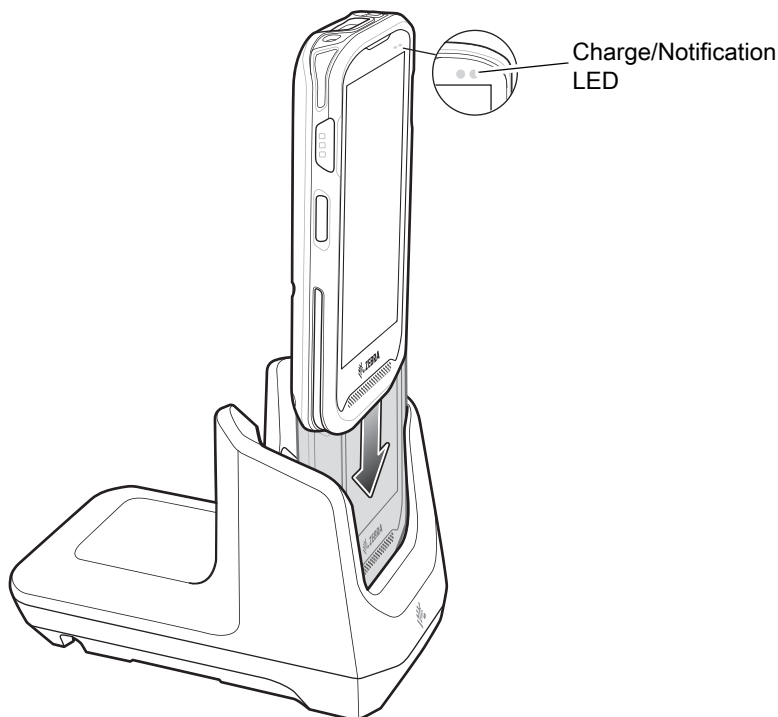
Figure 25 Battery Charging
