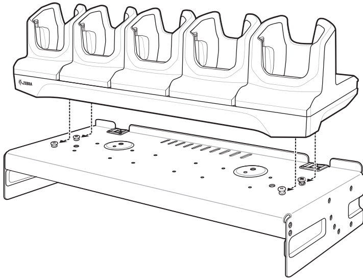
Figure 52 Align Cradle on Studs
