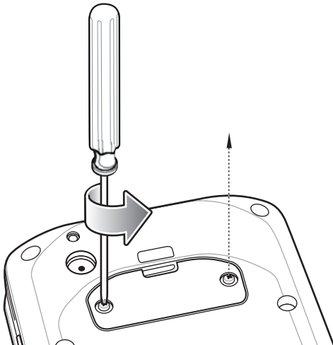
Figure 17 Remove Access Door
