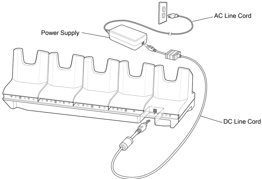
Figure 40 5-Slot Charge Only Cradle Setup
