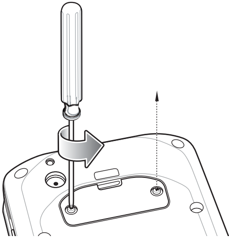
Figure 1 Remove Access Door
