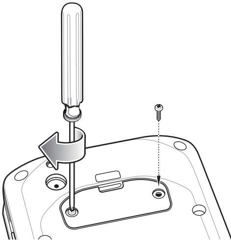
Figure 20 Replace Access Door
