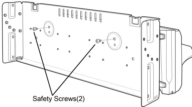
Figure 53 Secure Cradle
